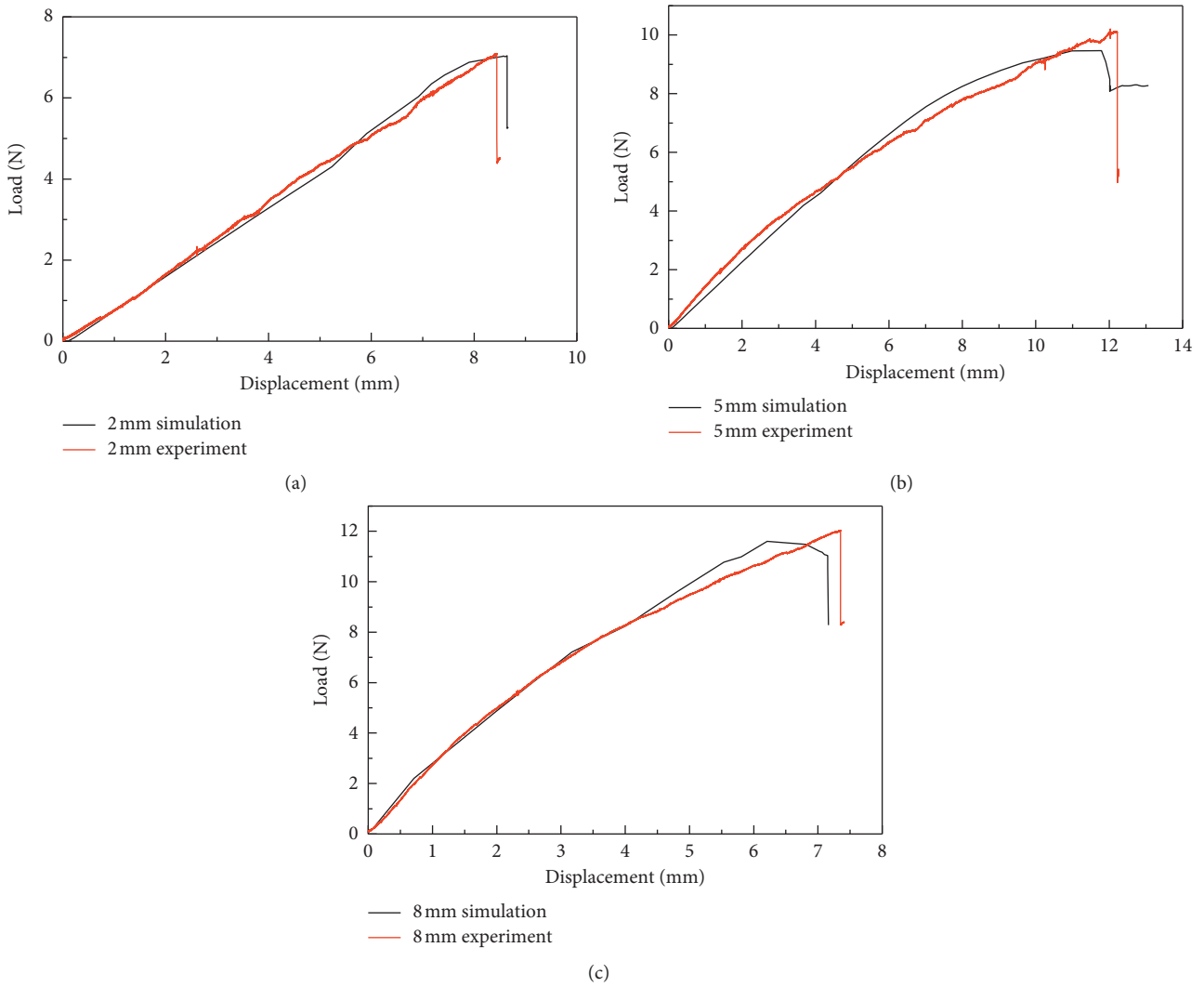
FIGURE 10: The load-displacement cure of the multilayer composite structure about solar cells.
