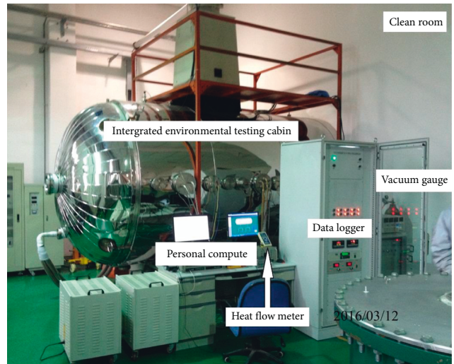
FIGURE 13: Photograph of the experimental apparatus.
