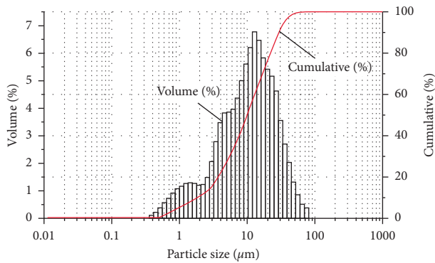
FIGURE 2: The grain-size distribution curve of cement.
