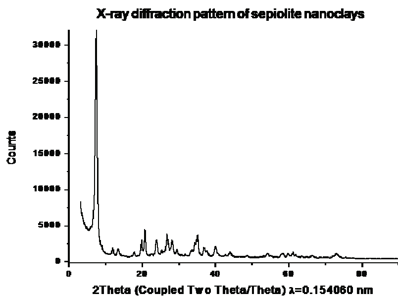
Figure S1. X-ray diffraction pattern of clinoptilolite and sepiolite nanoclays. The pics correspond to the diffraction planes. Sepiolite nanoclays match perfectly with the pattern of the PDF-2 database from the International Centre for Diffraction data and Clinoptilolite NC correspond to a Nickel Ammonium Aluminium Silicon Hydroxide Oxide Hydrate.
