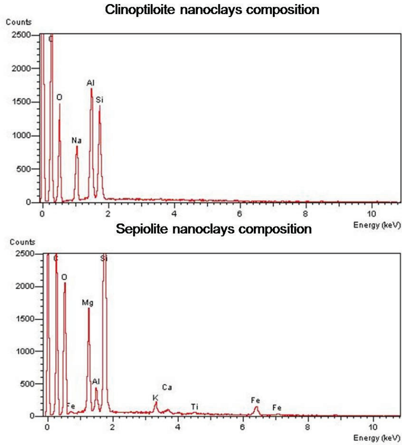
Figure S2. Microanalysis of clinoptilolite and sepiolite nanoclays determined by SEM. Metal content of nanoclays was the same that data found by atomic absorption.
