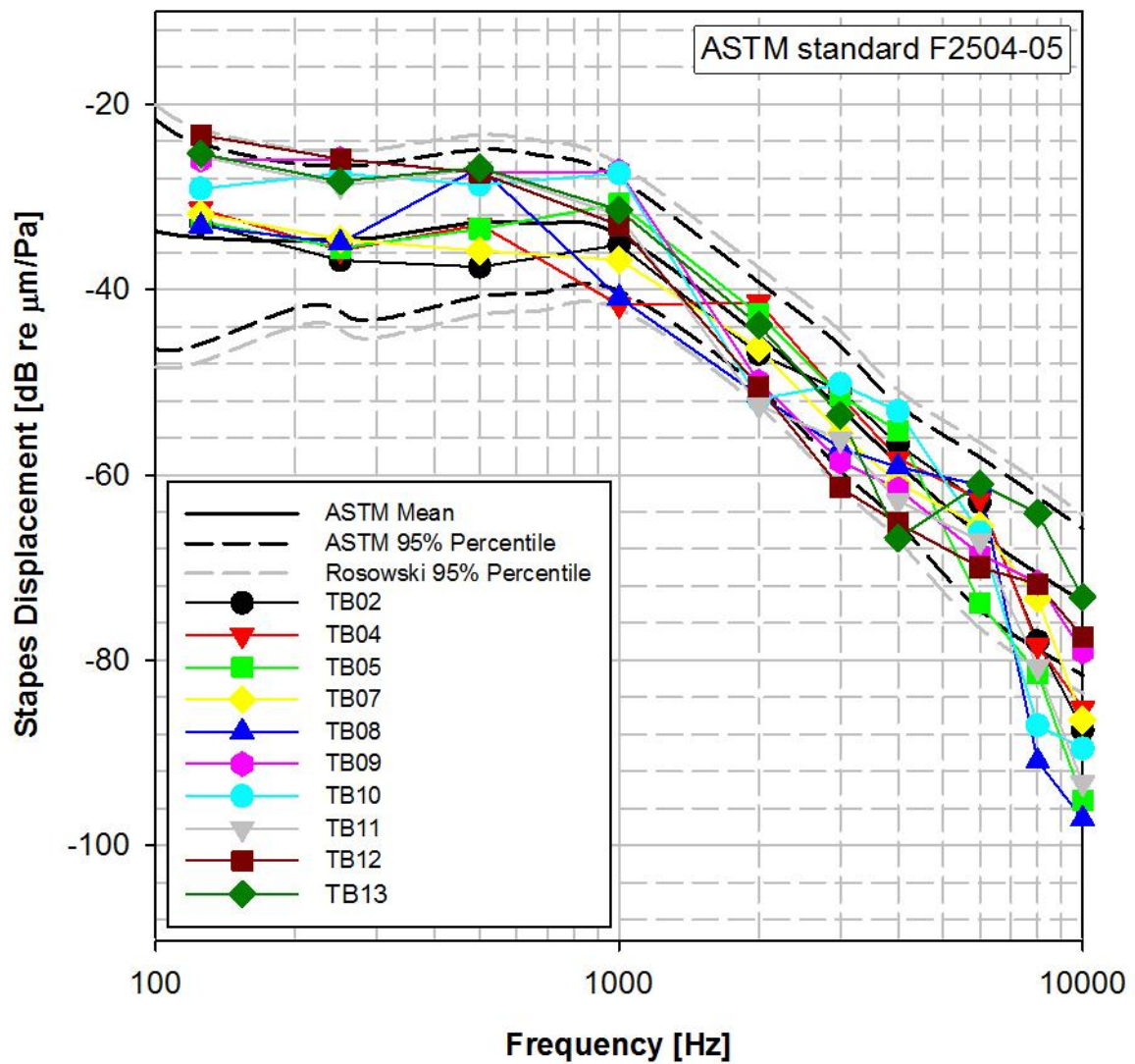
384 Figure 6: SFP displacement amplitudes in response to acoustic stimulation of the 385 tympanic membrane (~94 dB SPL) of ASTM [17] compliant temporal bones (n=10). 386 Black dashed lines represent the ASTM acceptance range and gray dashed lines 387 represent the extended acceptance range [14] used in this study.
