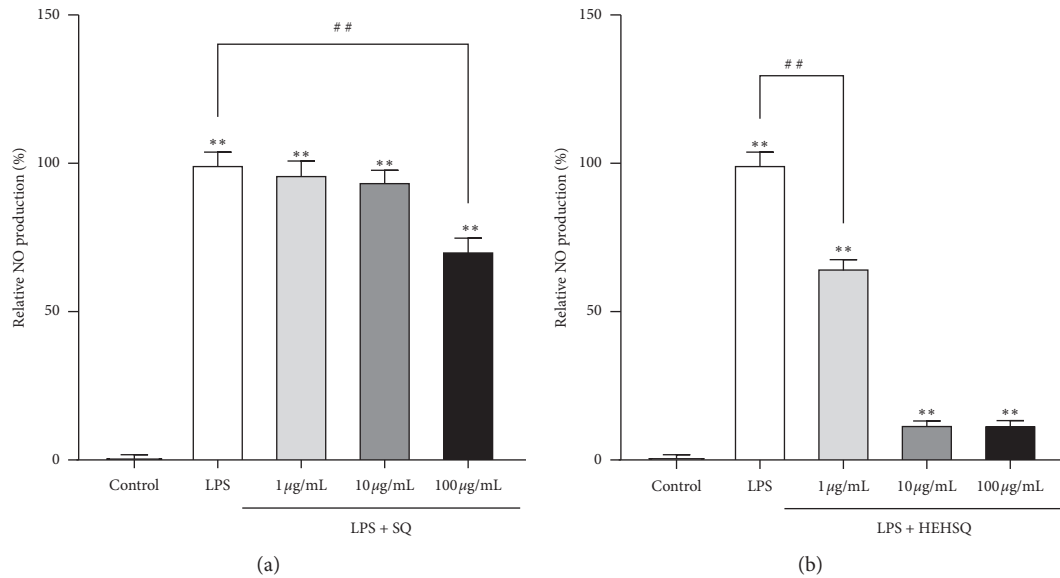
FIGURE 3: Effects of (a) squalene (SQ) and (b) 2-(2-hydroxyethoxy)-3-hydroxysqualene (HEHSQ) on LPS-stimulated NO production in RAW264.7 cells. Cells were treated with SQ or HEHSQ at 1, 10, and 100 \mu\text{g}/\text{mL} for 24 h. Subsequently, cells were activated with LPS (1 \mu\text{g}/\text{mL} ) for 12 h. The amount of NO production was measured by the Griess reaction. Values are expressed as the mean \pm SD of triplicate experiments and are expressed relative to the percentage of control LPS (-). The mean value that is significantly different from that of the control LPS (-) group is indicated as ** P < 0.01 . The mean value that is significantly different from that of the control LPS (+) group is indicated as ## P < 0.01 .
