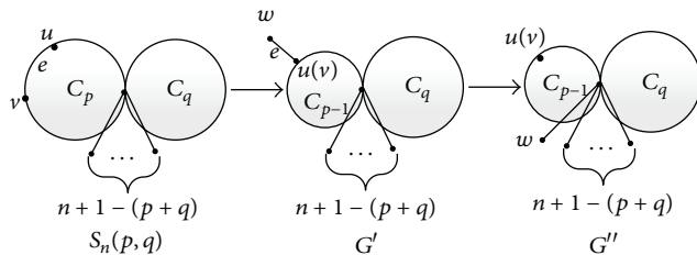
FIGURE 6: Graph transformations.
