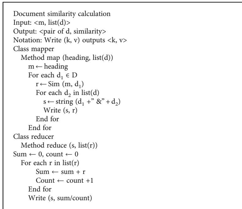
ALGORITHM 3: Algorithm of MapReduce-based document similarity calculation.
