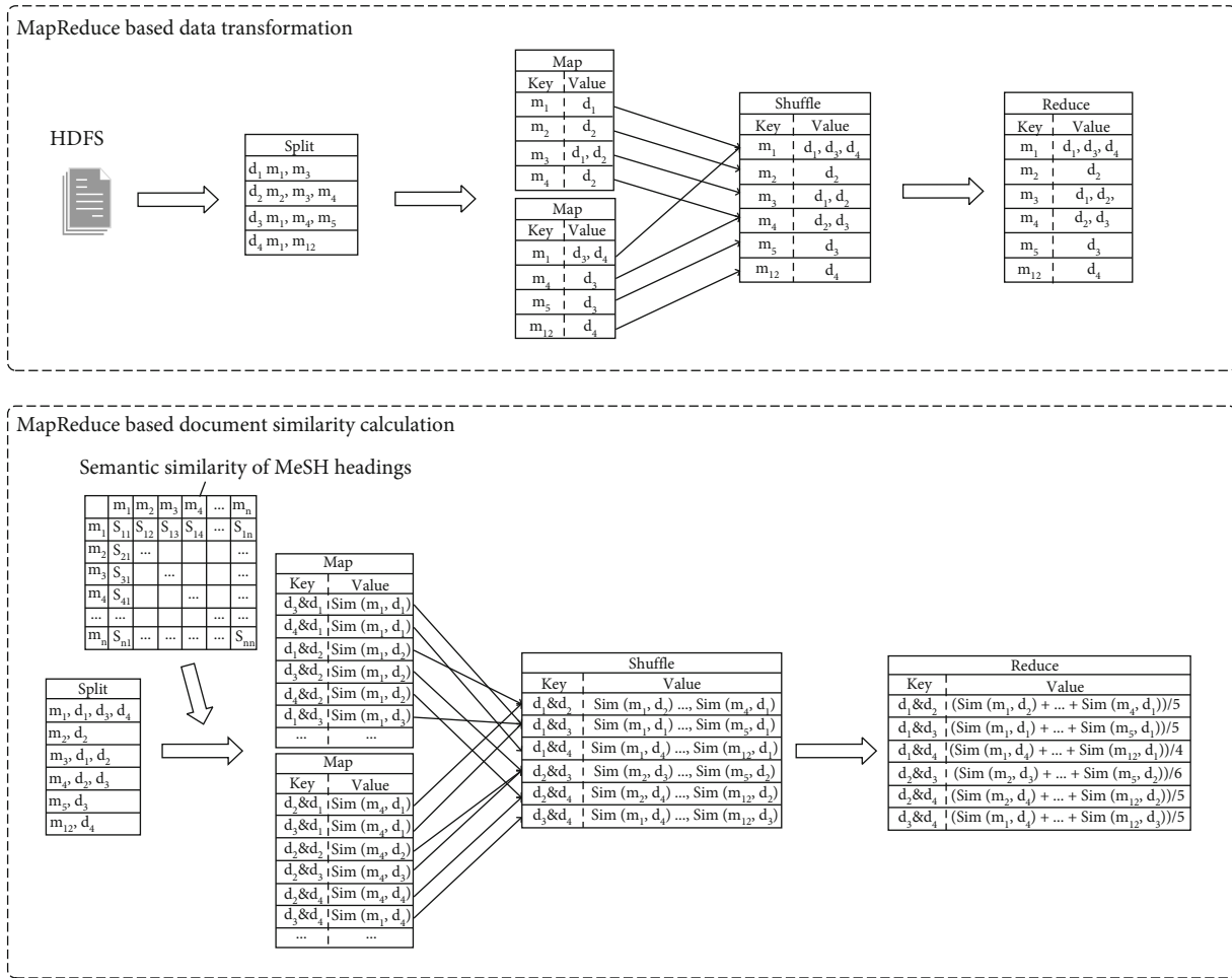
FIGURE 2: An example of MapReduce-based data transformation and semantic similarity calculation.
