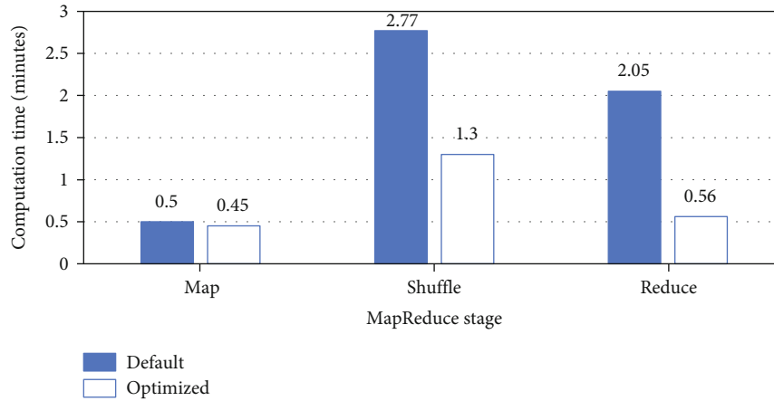
FIGURE 3: The result of MapReduce job optimization.
