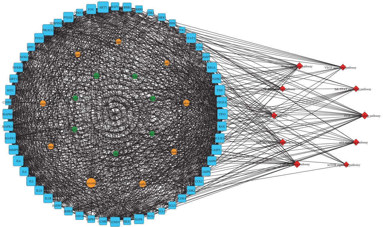
FIGURE 2: Herb-compound-target-signaling pathway network of BSJPD. Notes. The green octagon nodes represent herbs, the orange ellipse nodes represent compounds, the blue square nodes represent targets, and the red diamond nodes represent signaling pathways. The sizes of the nodes are illustrated from large to small in descending order of degree values. BSJPD, Bushen-Jianpi decoction.
