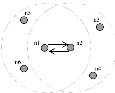
Figure 1. Collision domain of two communicating sensors.
