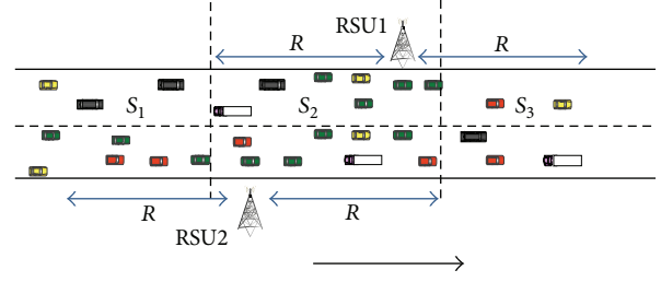
FIGURE 2: The two RSUs' scene.
