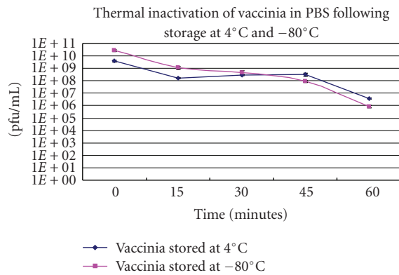
FIGURE 3: The inactivation of vaccinia virus stored at 4°C and -80°C for one week and inactivated at 56°C in PBS, pH 7.4.
