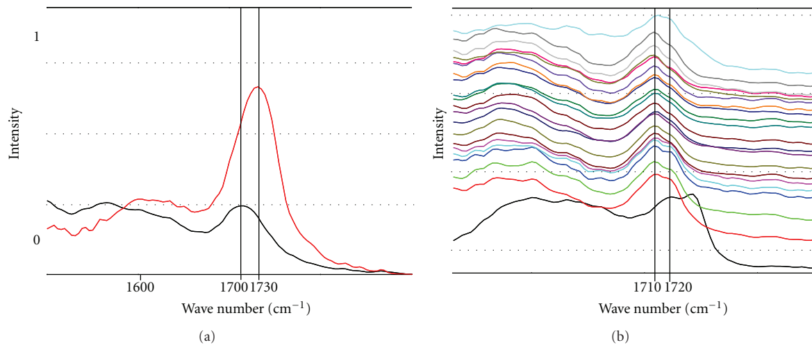
FIGURE 6: IR spectra. (a) IR spectrum of silane on \text{Al}_2\text{O}_3 . Shift of C=O peak; red graph: high silane concentration, black graph: low silane concentration. (b) 20 IR spectra in the range of 1530 to 1850 \text{cm}^{-1} . Each spectrum represents a measurement point on a line scan, measured analogously to the in Figure 3(c) described system (Topmost spectrum = top plane; lowermost spectrum = bottom plane; used silane concentration 0.36%).
