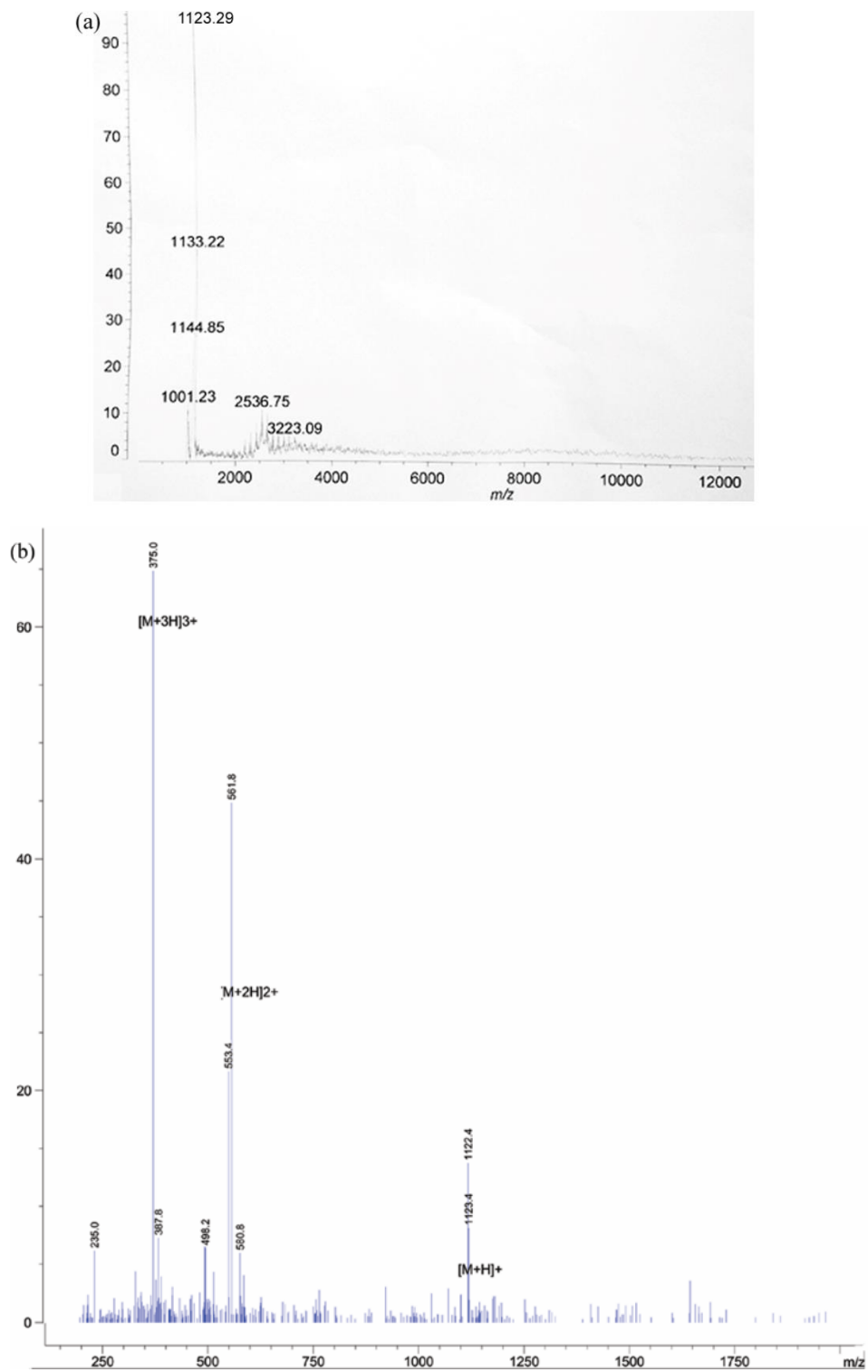
Fig. S1 MALDI-TOF-MS (a) and ESI-MS (b) spectrum of the peptide P2
