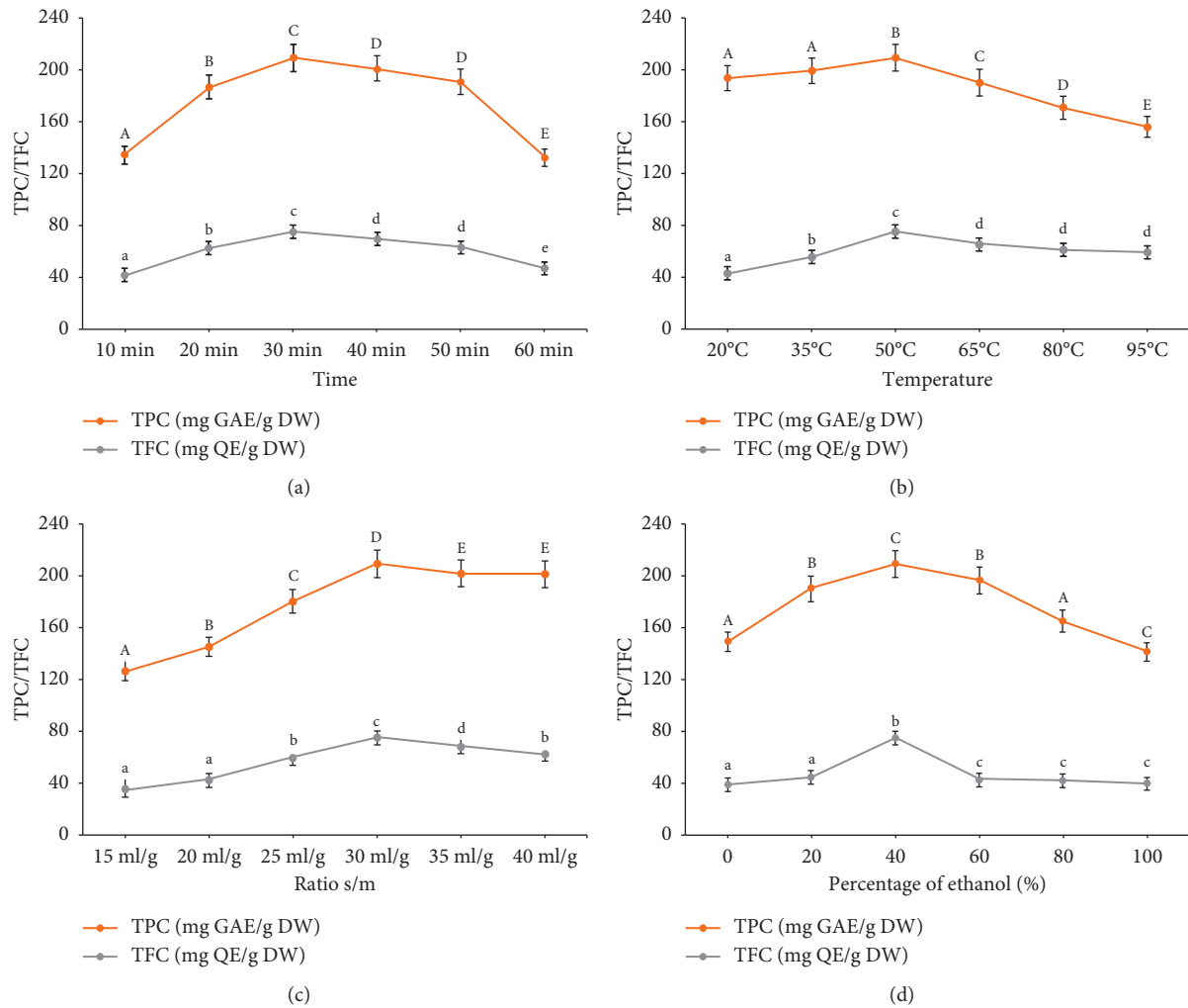
FIGURE 2: Effect of extraction time (a), temperature (b), ratio s/m (c), and ethanol (%) (d) on total phenol and flavonoid contents from Eucalyptus marginata L. leaves using the ultrasound-assisted extraction method.
