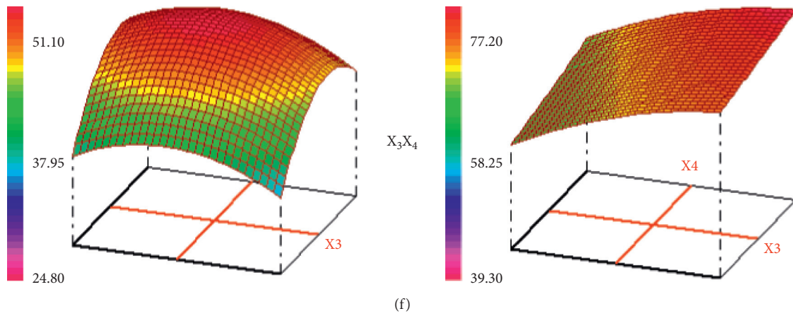
FIGURE 4: Response surface plot of TFC (mg QE g -1 DW) of Eucalyptus marginata leaves extracts as a function of time, temperature, ratio s/m, and ethanol concentration obtained by maceration and ultrasound-assisted extraction methods. The extraction time (min, X_1 ), temperature (°C, X_2 ), liquid/solid ratio (ml/g, X_3 ), and ethanol concentration (% , X_4 ).
