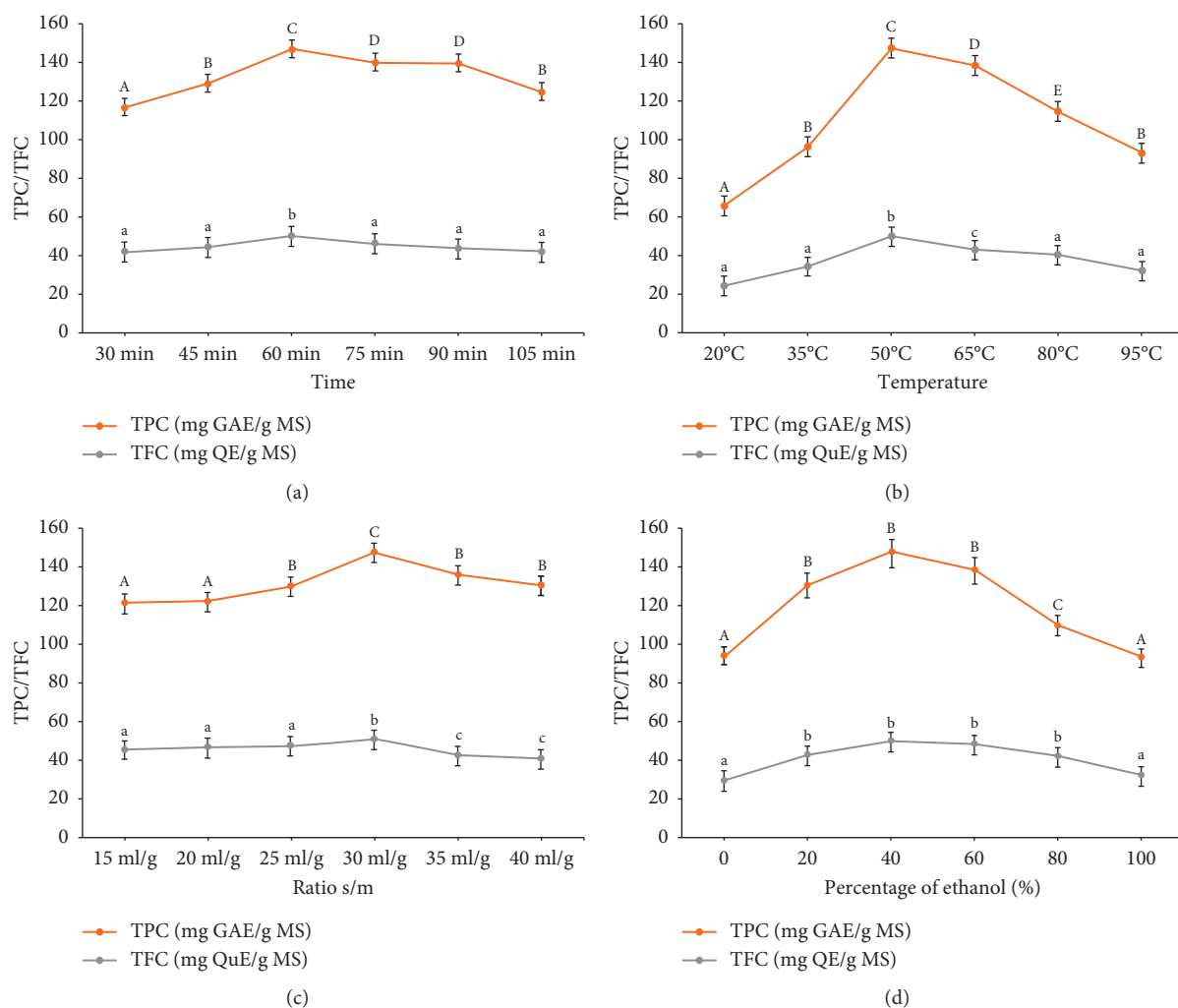
FIGURE 1: Effect of extraction time (a), temperature (b), ratio s/m (c), and ethanol (%) (d) on total phenol and flavonoid contents from Eucalyptus marginata L. leaves using the maceration extraction method.
