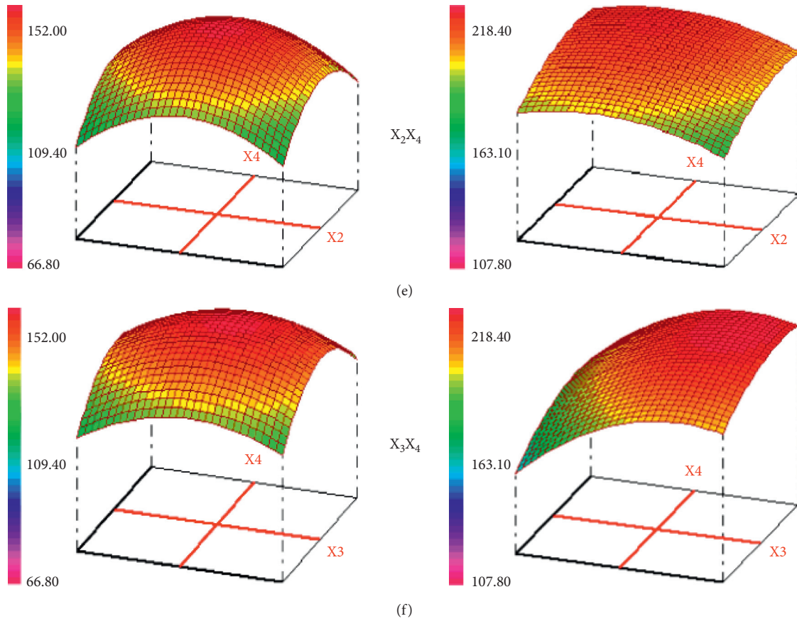
FIGURE 3: Response surface plot of TPC (mg GAE g -1 DW) of Eucalyptus marginata leaves extracts as a function of time, temperature, ratio s/m, and ethanol concentration obtained by maceration and ultrasound-assisted extraction methods. The extraction time (min, X_1 ), temperature (°C, X_2 ), liquid/solid ratio (ml/g, X_3 ), and ethanol concentration (%), X_4 ).
