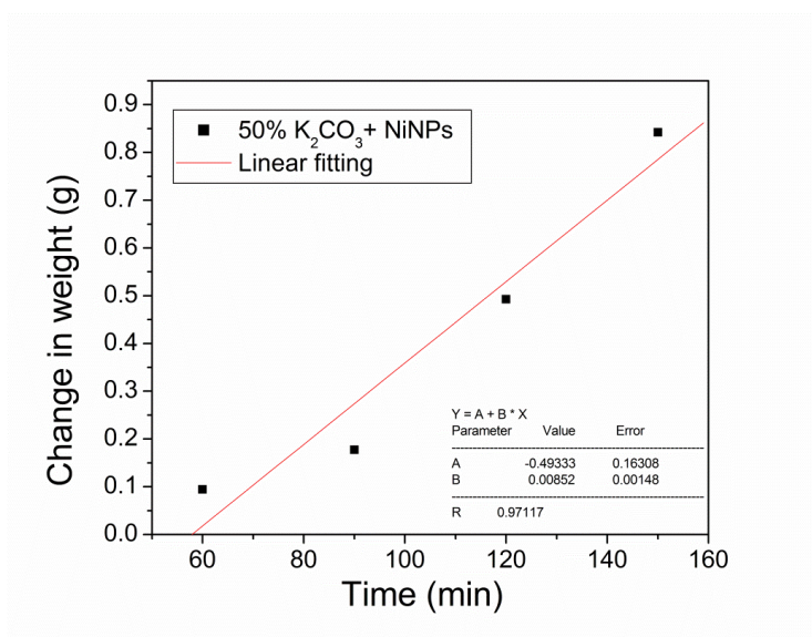
Figure S2: CO 2 absorption in 50% potassium carbonate solution in presence of NiNPs using liner fit.
