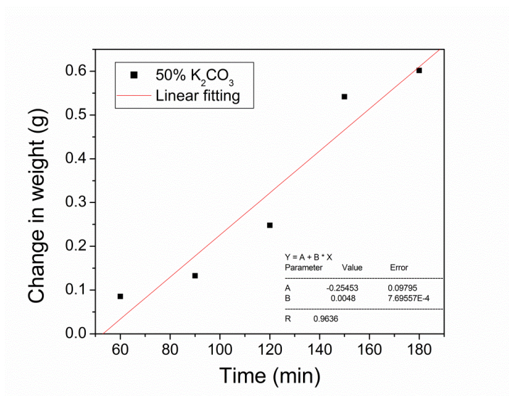
Figure S1: CO 2 absorption in 50% potassium carbonate solution using liner fit.
