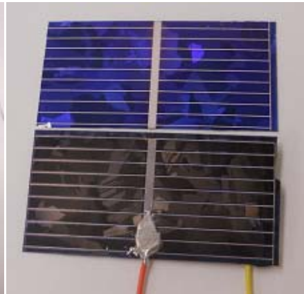
Silicon nitrate coated polycrystalline Si solar cell(top) and Blackened polycrystalline Si solar cell(bottom)
