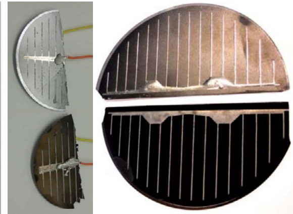
Blackened KOH textured single crystal Si solar cell(top) and control(bottom)
