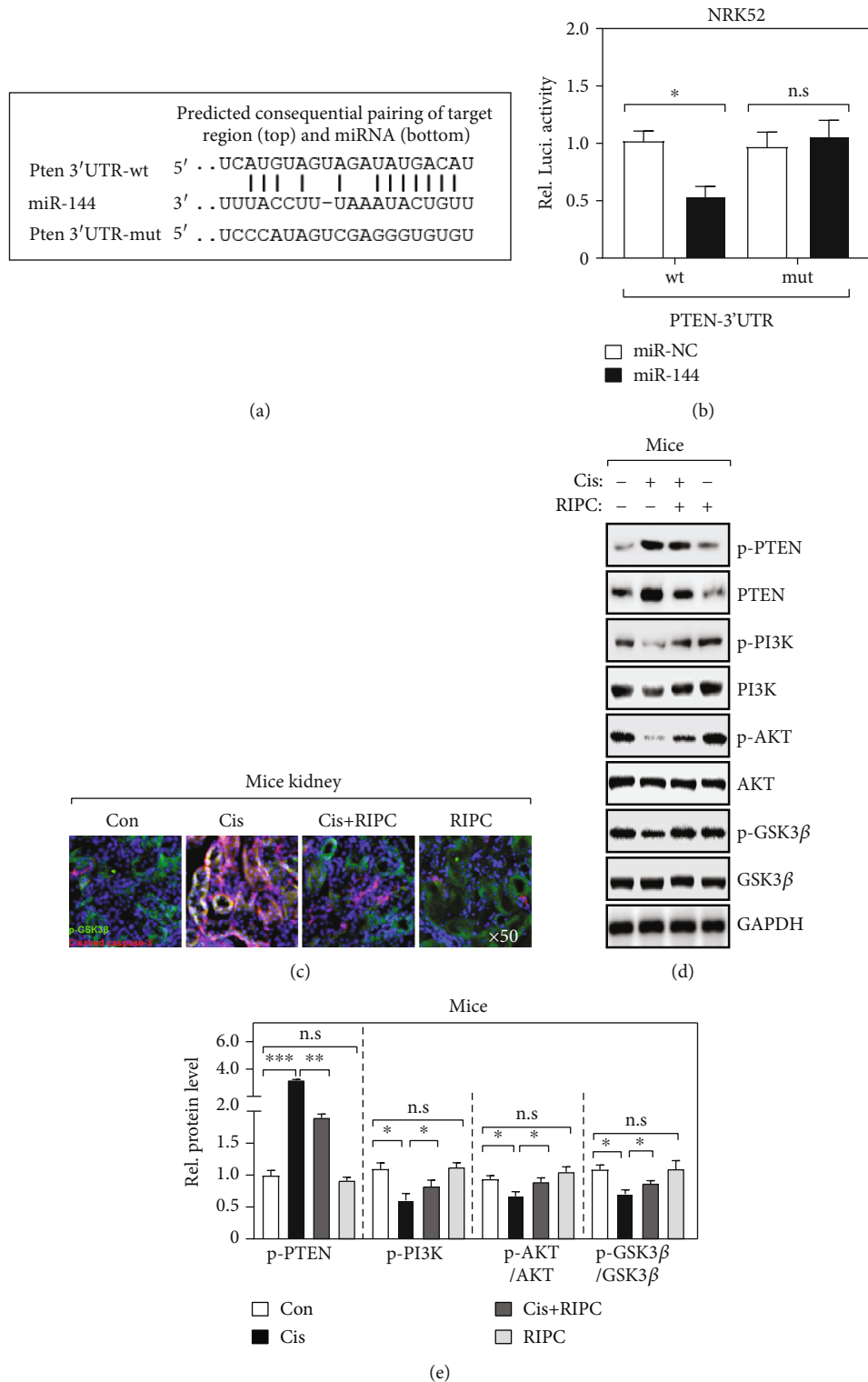
FIGURE 3: MiR-144 activates the AKT/GSK3 \beta pathway by directly targeting PTEN (a) The sequence alignment of miR-144 and the 3'-UTR of PTEN mRNA. Wild-type (wt) and mutant (mut) sequences were used in (b). (b) Luciferase activities determined the binding between miR-144 and 3'-UTR of PTEN. NRK52 cells were cotransfected with the indicated plasmids. Each firefly luciferase activity was normalized by the cotransfected Renilla luciferase activity. n = 6 ; * P < 0.05 ; n.s: no significance in statistic. (c) Representative confocal image of immunofluorescence staining with p-GSK3 \beta and cleaved caspase-3 in kidney sections. (d, e) Western blot determined the indicated protein level (d) and their quantification (e). n = 6 ; * P < 0.05 ; ** P < 0.01 ; *** P < 0.001 ; n.s: no significance in statistic.
