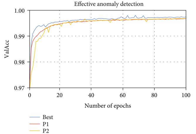
FIGURE 2: Validation accuracy versus the number of epochs for the binary classification for the best performing permutations of the hyperparameters.
