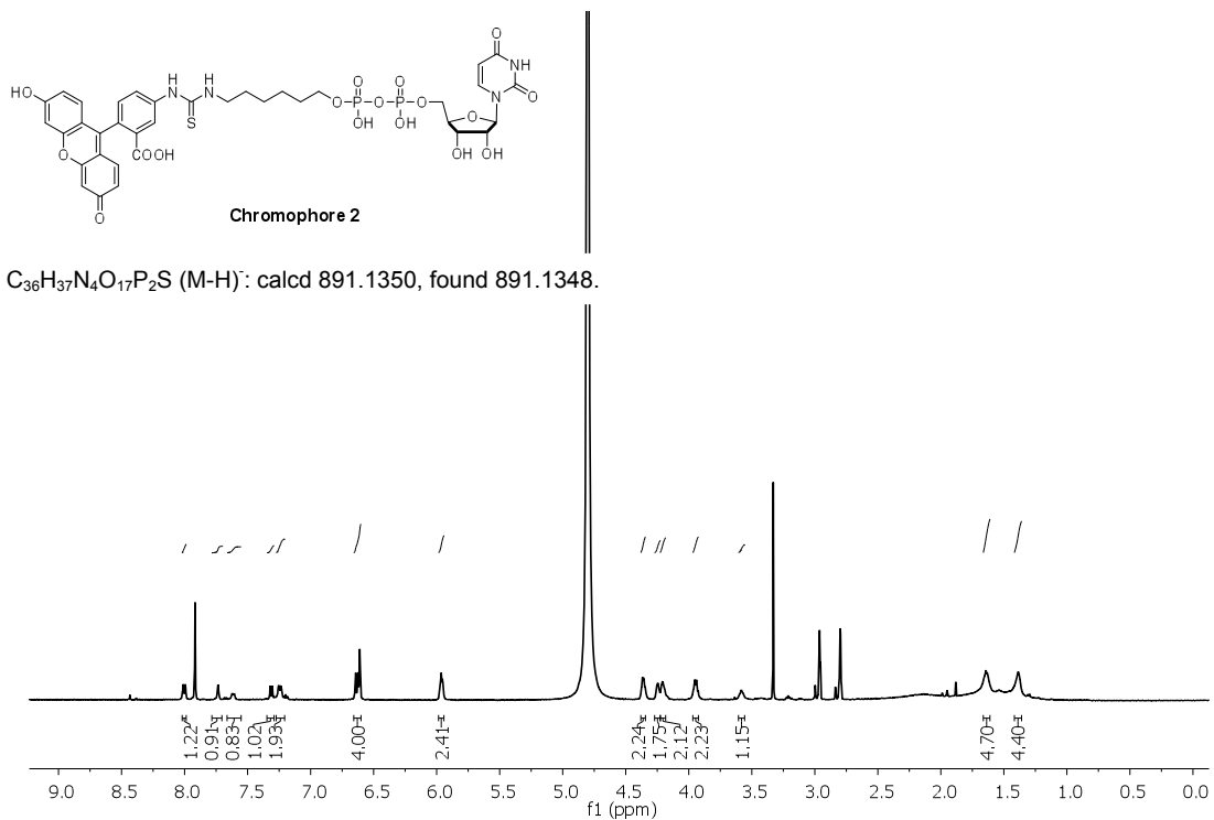
Figure S3. ^1\text{H} NMR spectrum and high-resolution mass spectrum of chromophore 2
