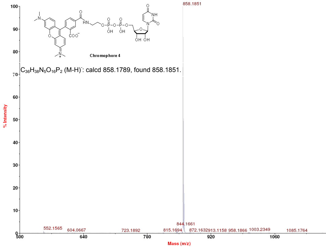
Figure S5. High-resolution mass spectrum of chromophore 2
