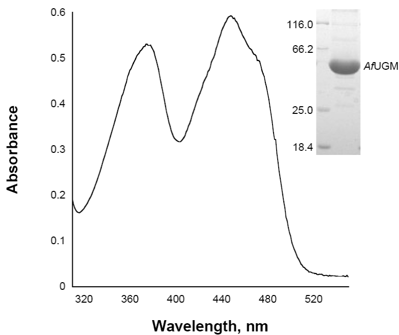
Figure S1. UV-visible spectrum and SDS-PAGE of Af UGM
