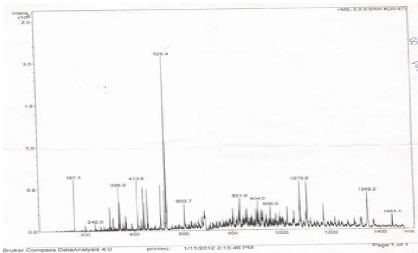
ESI-MS of complex 3
