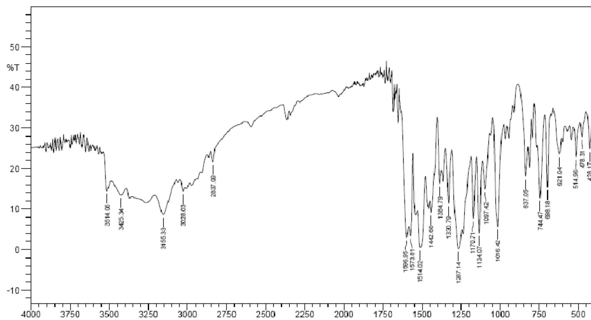
IR Spectra of complex 3
