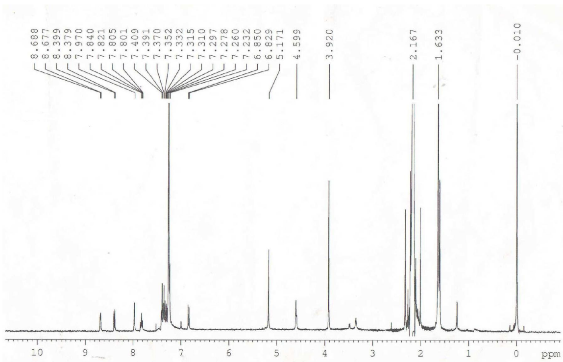
1 H NMR spectra of complex 2
