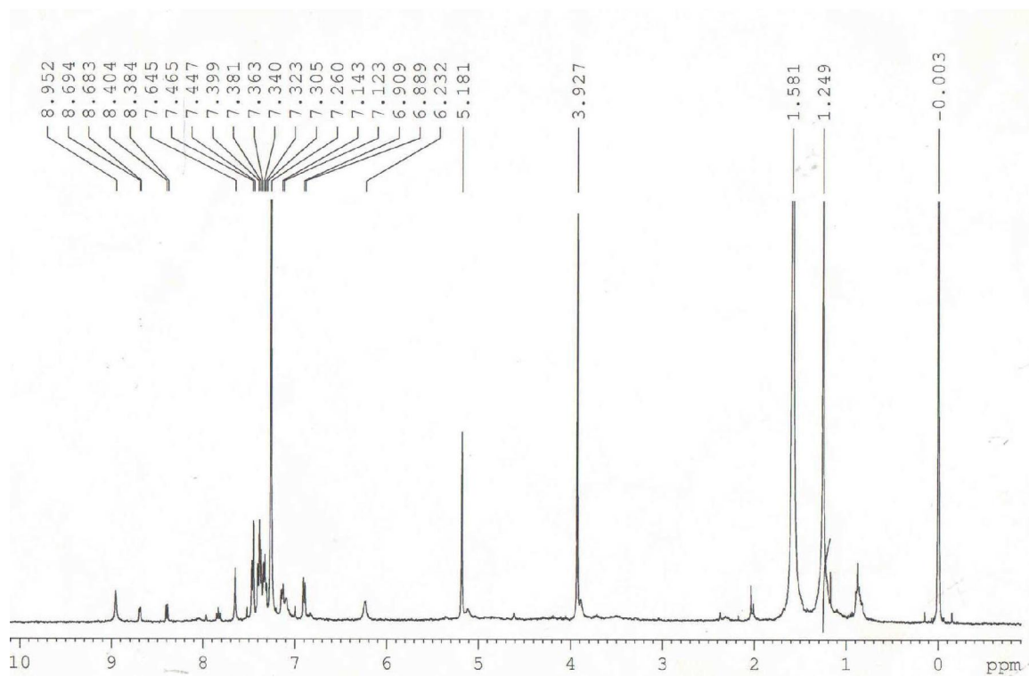
1 H NMR spectra of complex
