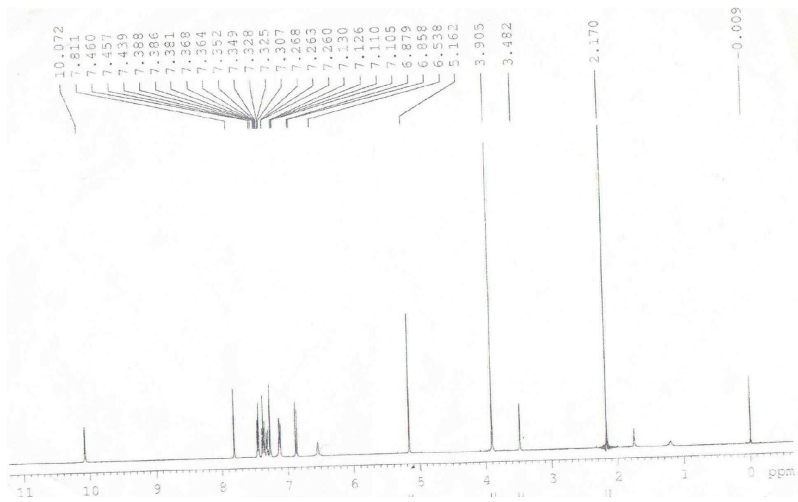
^1\text{H} NMR spectra of complex 1
