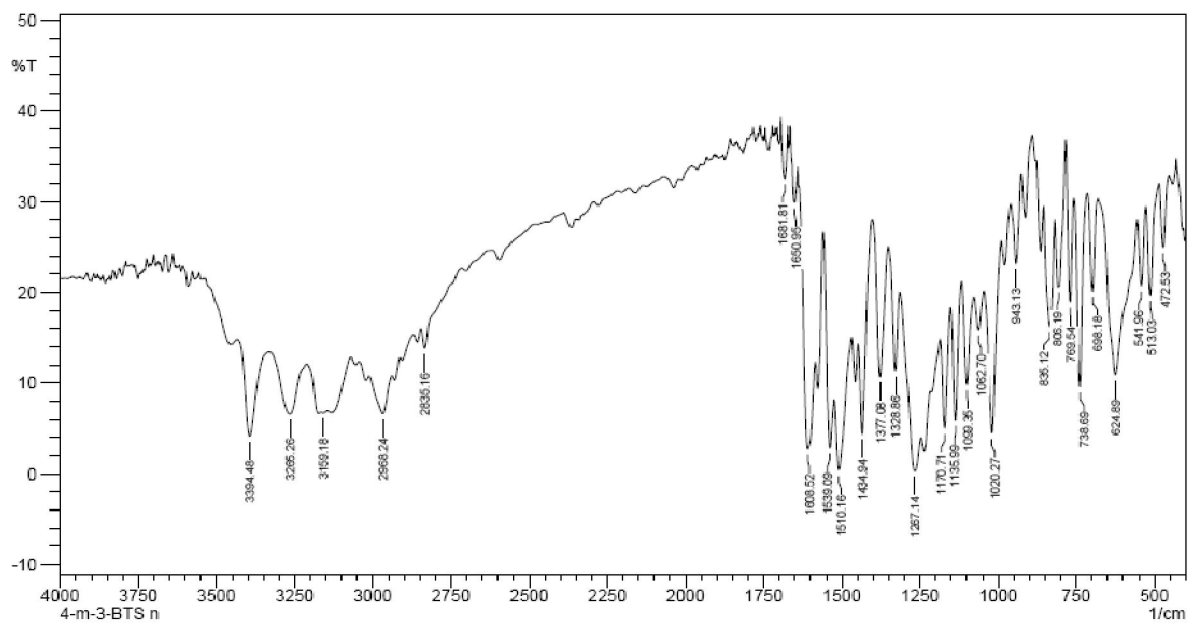
IR Spectra of complex 1
