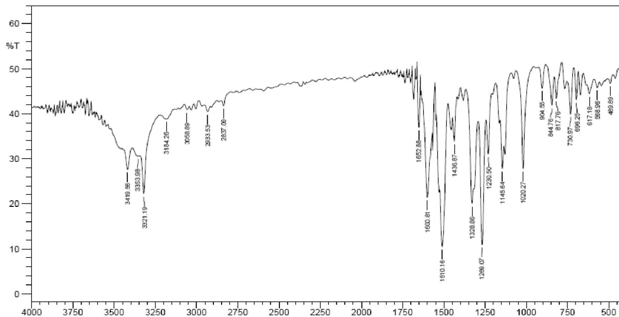
IR Spectra of complex 2
