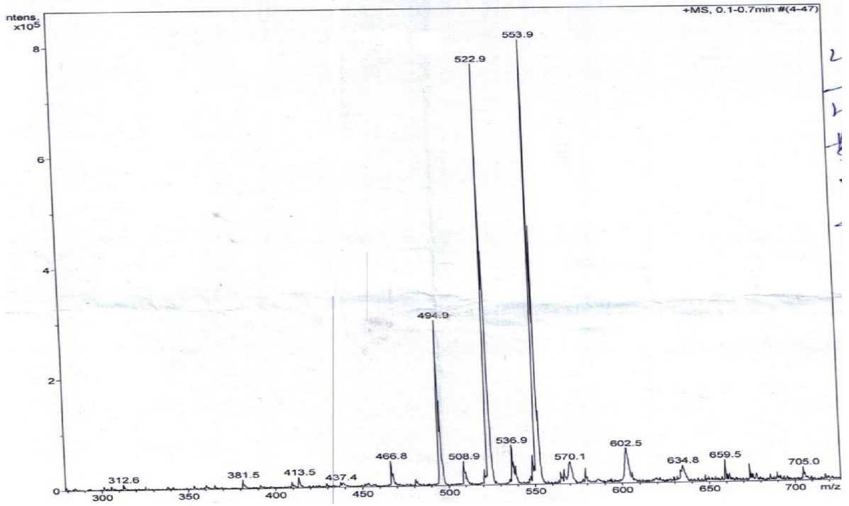
ESI-MS of complex 2
