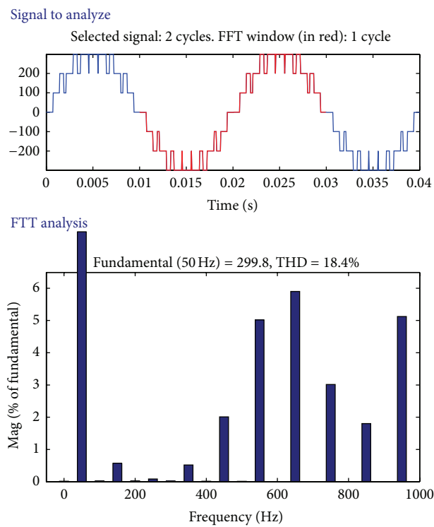
FIGURE 15: FFT analysis of proposed topology using APOD pwm.
