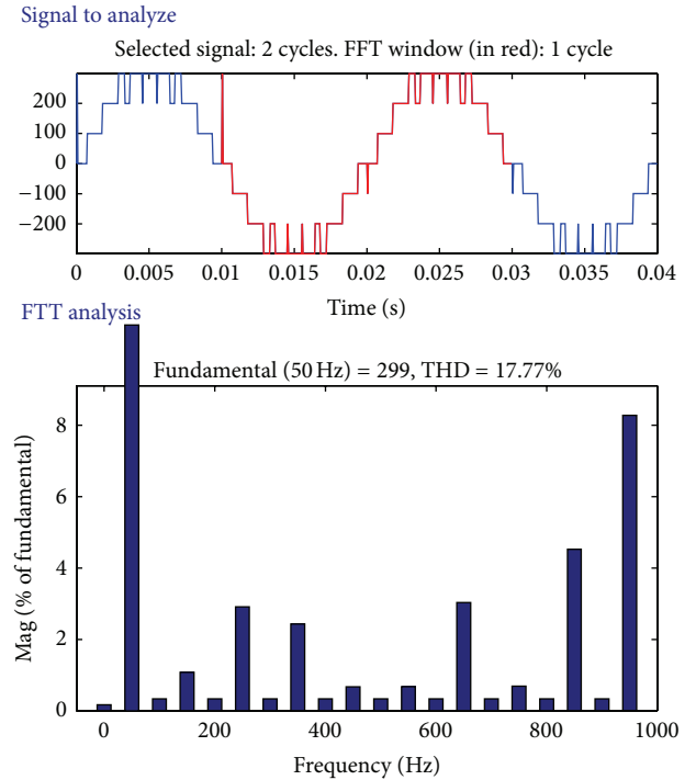
FIGURE 11: FFT analysis of existing 6-switch topology using POD pwm.
