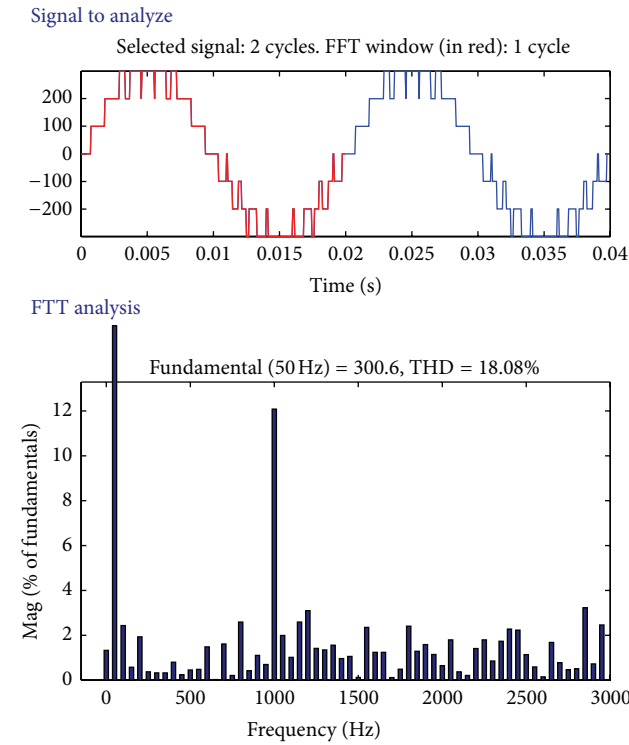
FIGURE 10: FFT analysis of existing 6-switch topology using PD pwm.
