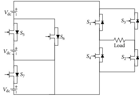
FIGURE 3: 7-level 7-switch topology.
