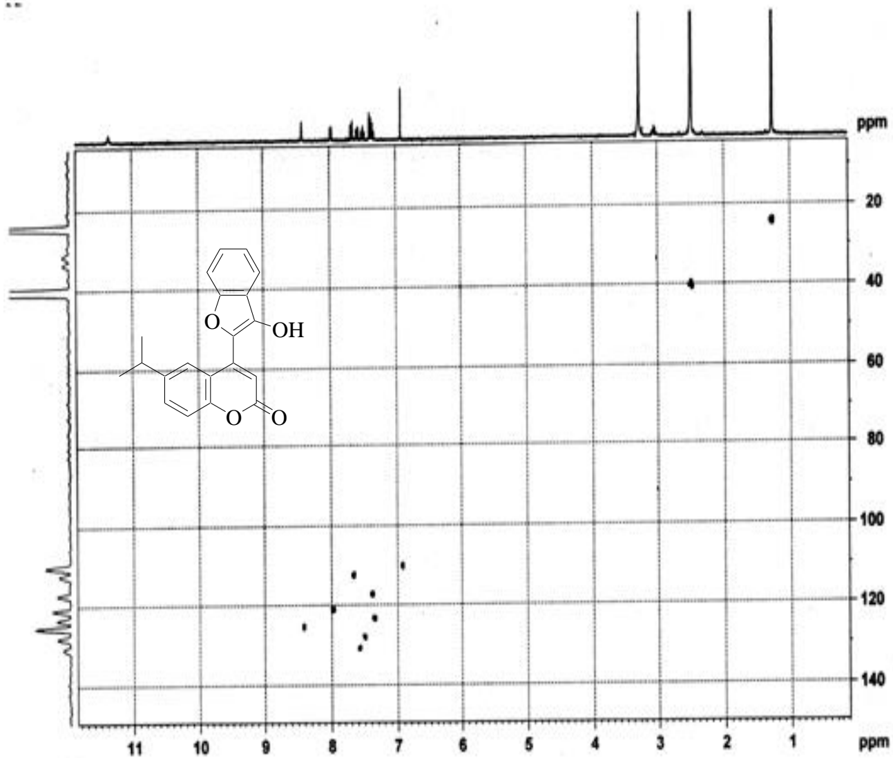
HSQC spectra of 3h
