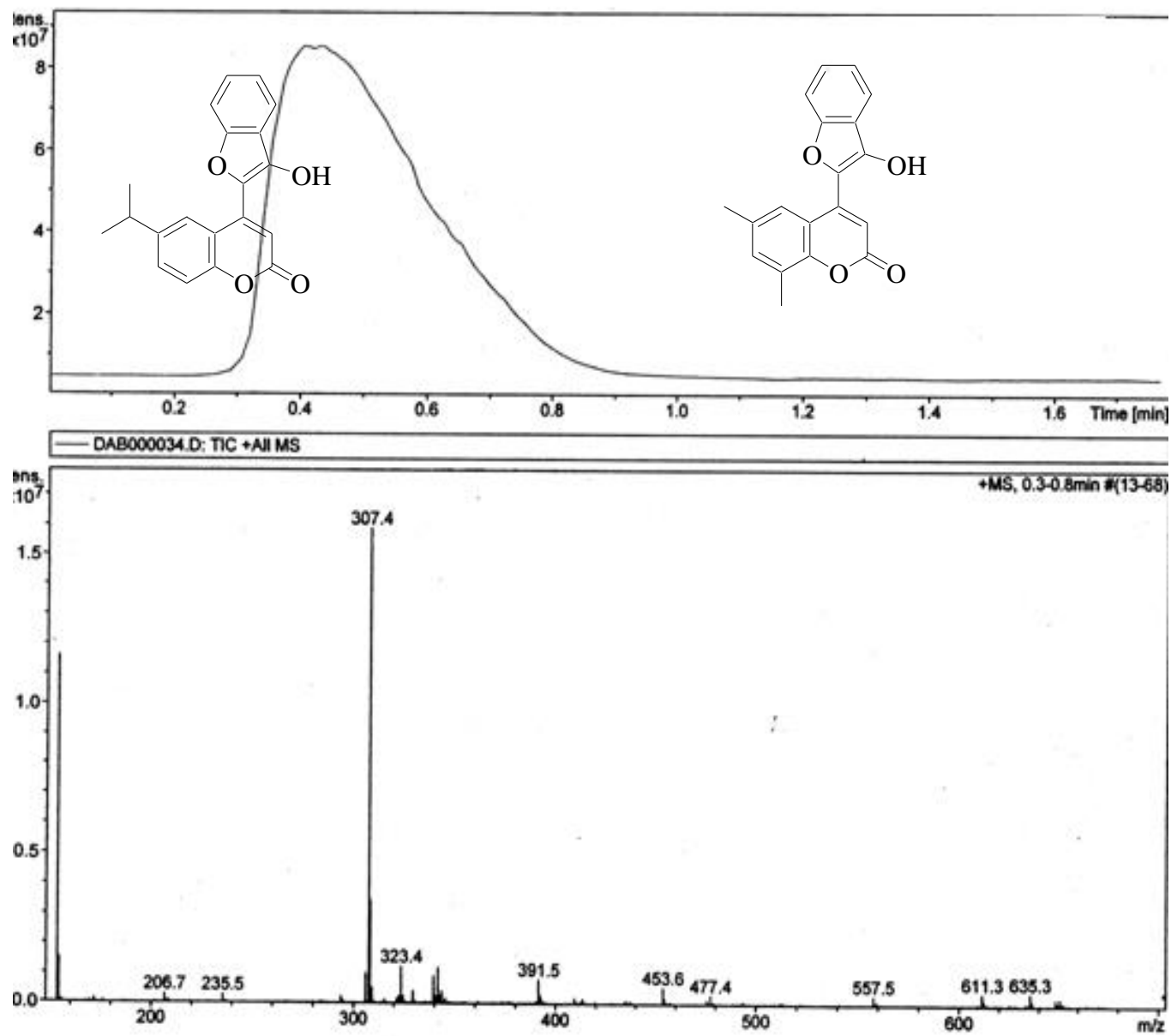
LC-Mass spectra of 3g
