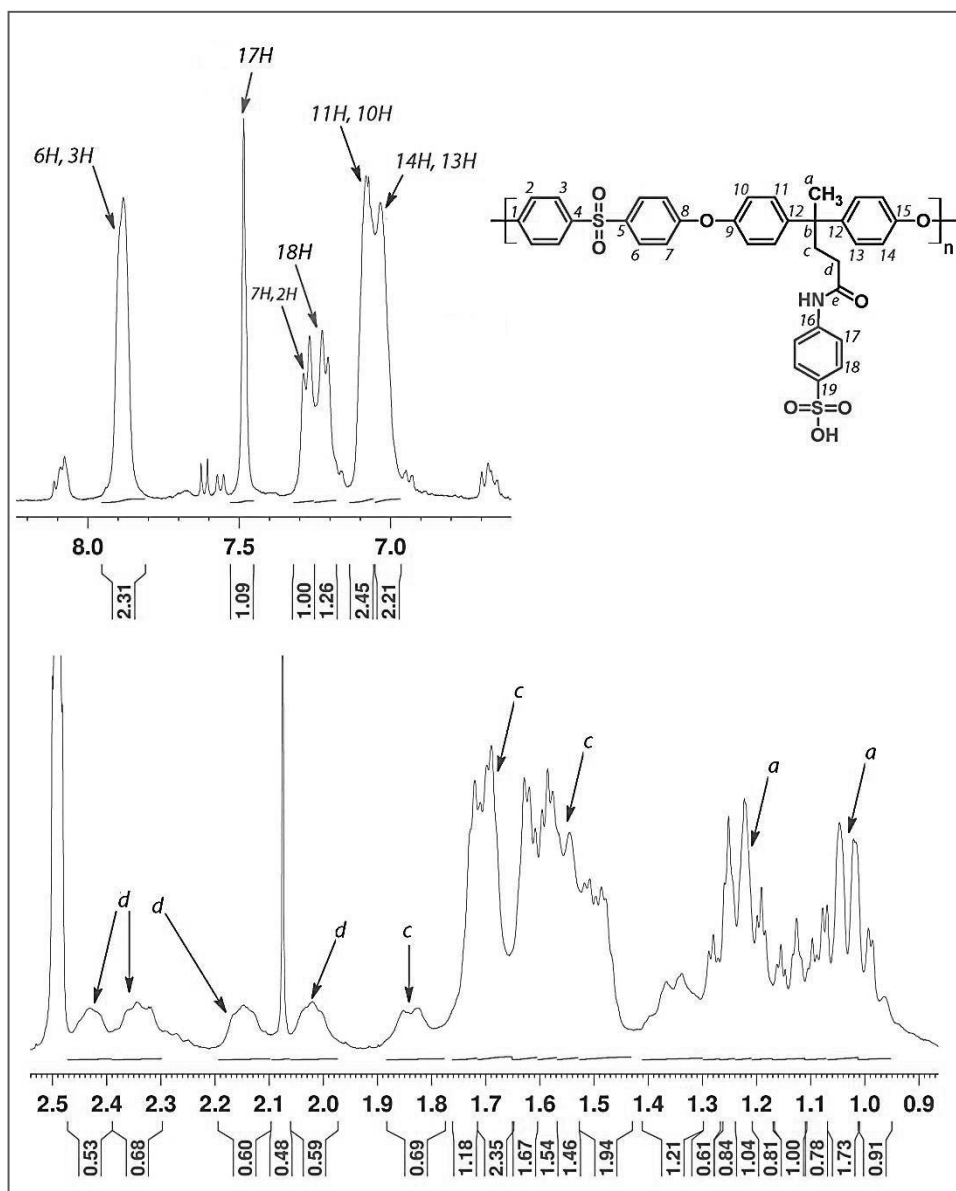
Figure S1. ^1\text{H} NMR ( \text{DMSO-d}_6 ) spectrum of PS-40
