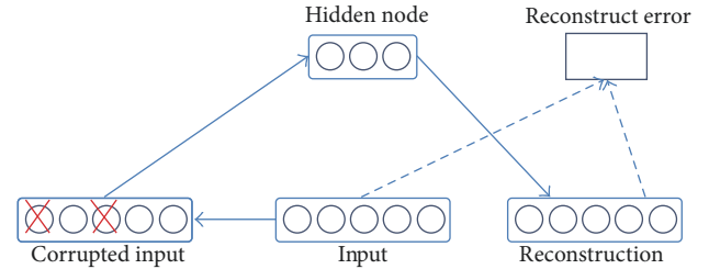
FIGURE 3: Denoising autoencoder [56].
