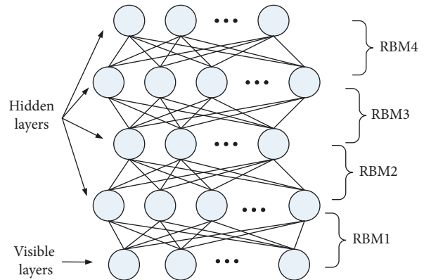
FIGURE 2: Structure of deep belief network.
