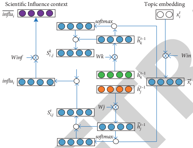
FIGURE 4: Scientific influence modeling based on semantic consistency.
