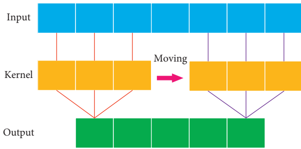
FIGURE 12: Diagram of one-dimensional convolutional neural networks.
