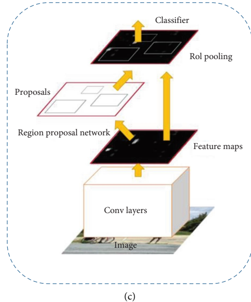
FIGURE 3: Faster RCNN series algorithm framework diagram [44, 55, 56]. (a) RCNN. (b) Fast RCNN. (c) Faster RCNN.
