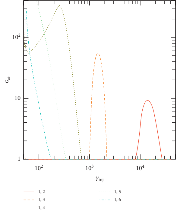
FIGURE 2: The growth factors G_{nk} of betatron oscillations amplitudes as function of gamma-factors of injected electrons \gamma_{\text{inj}} , calculated by formulas (20)–(25). G_{nk} are estimated for a capillary waveguide with the same parameters as in Figure 1, for the duration of electron acceleration \Delta\tau = \tau - \tau_0 = 0.2k_p L_{\text{ph}} (where \tau_0 = k_p L_{\text{inj}} indicates the start of acceleration; \tau_0 = 3800 \approx 0.093k_p L_{\text{ph}} in calculations). The growth factors are due to the beating of the modes with the numbers n, k indicated on the legend.
