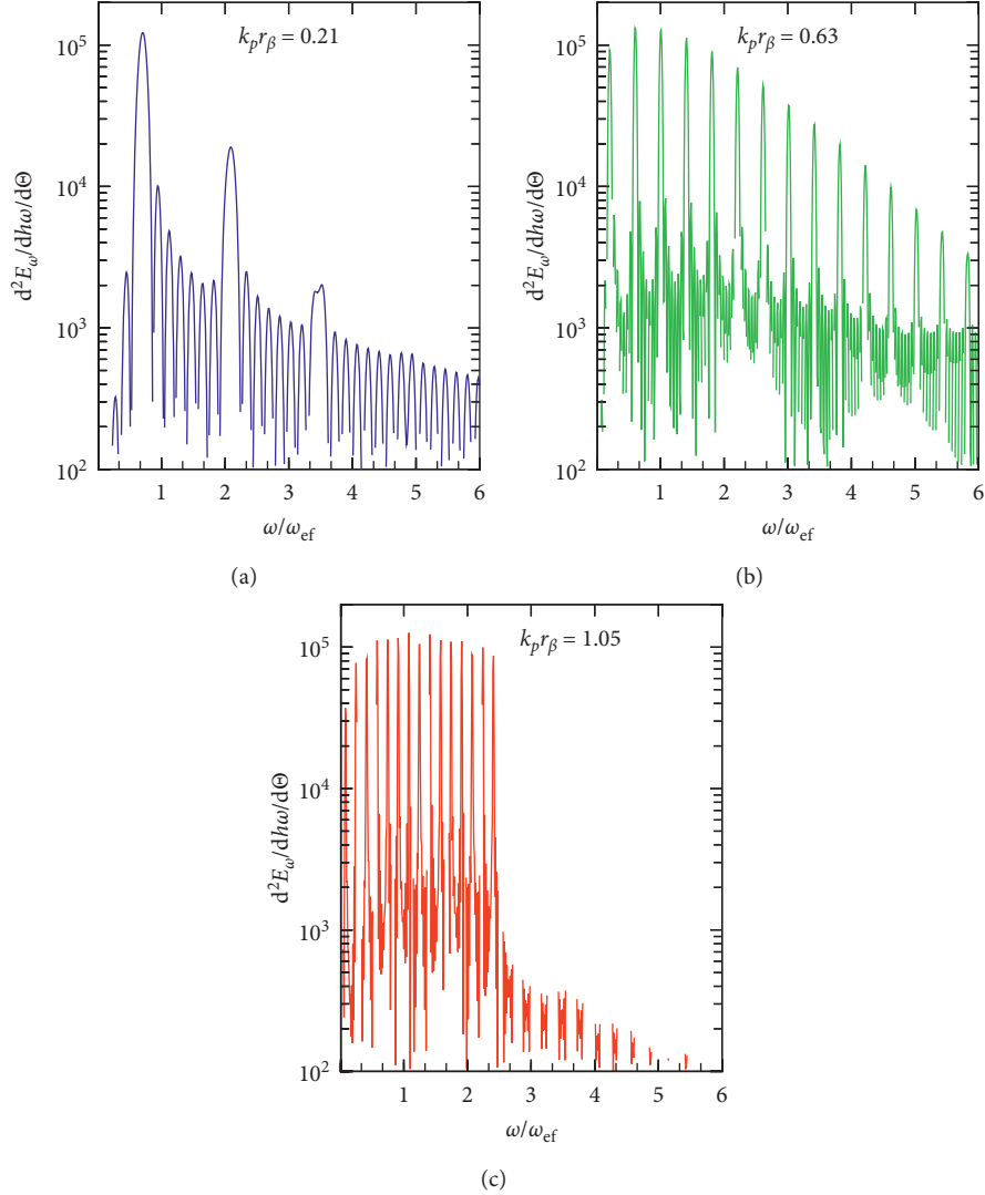
FIGURE 4: Energy d^2 E_\omega / (h d \omega d \Theta) , radiated in the direction 0z in a unit solid angle d\Theta in a unit frequency interval d\omega , during N_\beta = 4 betatron periods, for different k_p r_\beta = 0.21, 0.63, 1.05 (from left to right subfigures), \gamma_e = 2100 , and \Omega k_p L_{ph} = 60 . Other parameters are the same as in Figure 3. The characteristic quantum energy \hbar \omega_{ef} = 260 eV and the parameter a_\beta = 0.66, 1.99, 3.32 for given calculations with k_p r_\beta = 0.21, 0.63, 1.05 , respectively.
