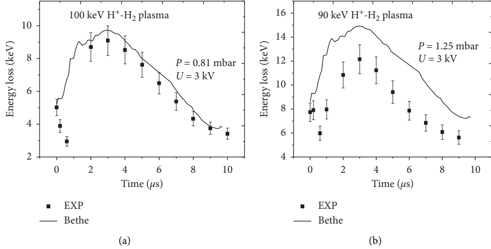
FIGURE 3: Energy losses of protons penetrating through hydrogen gas discharging plasma. (a) 100 keV proton in plasma (the initial gas pressure was about 0.81 mbar, and the voltage was 3 kV); (b) 90 keV proton in plasma (the initial gas pressure was about 1.25 mbar, and the voltage was 3 kV). The symbols represent experimental data. The solid line represents the theoretical predictions of the Bethe model with Z_{\text{eff}} = 1 .
