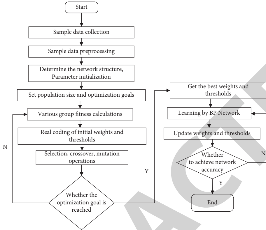
FIGURE 3: Flowchart of the optimized BP algorithm.
