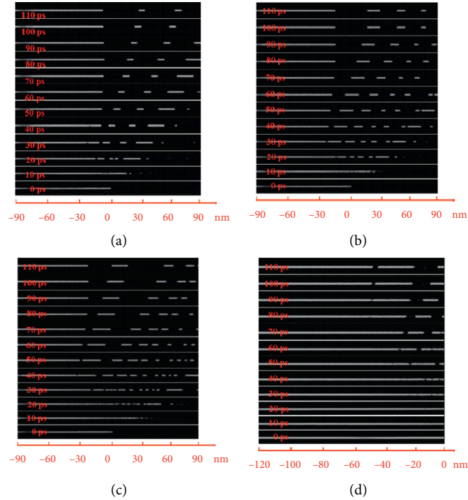
FIGURE 5: Schematic diagram of atomic snapshots at different energy densities: (a) 3188 \text{ J/m}^2 , (b) 4782 \text{ J/m}^2 , (c) 6377 \text{ J/m}^2 , and (d) 7971 \text{ J/m}^2 .
