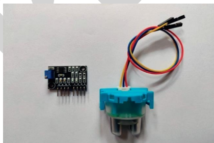
FIGURE 8: Water turbidity sensor module.
