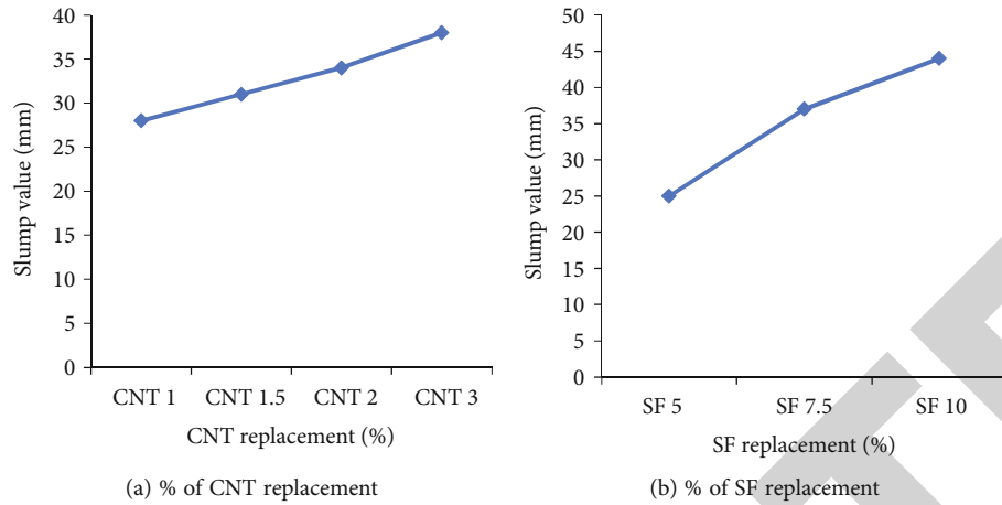
FIGURE 2: Variation of slump value.
