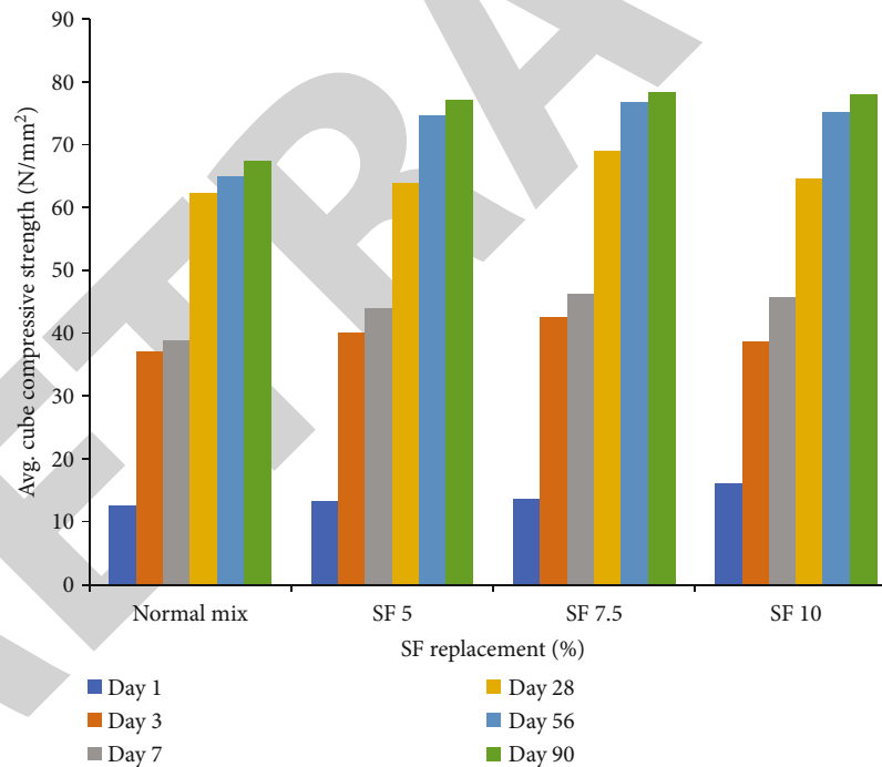
FIGURE 6: Fluctuation of compressive strength for % of SF replacement.
