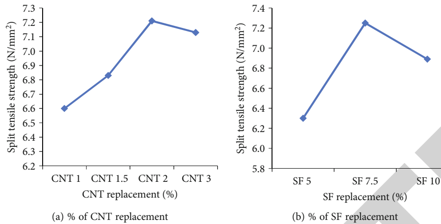
FIGURE 7: Split tensile strength variation at the 28 th day.
