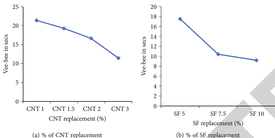
FIGURE 4: Variation of vee-bee consistometer.
