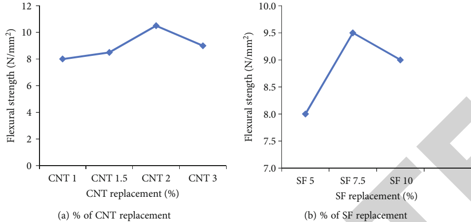
FIGURE 8: Variation of flexural strength at the 28 th day.
