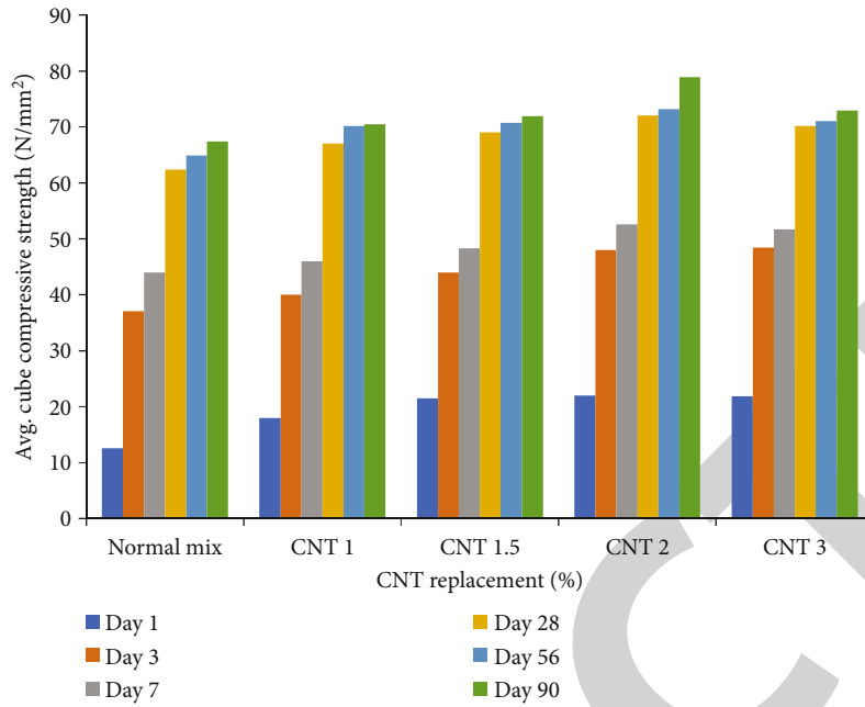
FIGURE 5: Fluctuation of compressive strength for % of CNT replacement.
