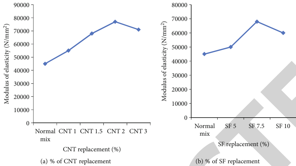
FIGURE 10: Variation of modulus of elasticity.
