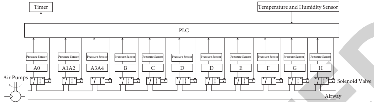
FIGURE 13: Airbag mattress pneumatic device.
