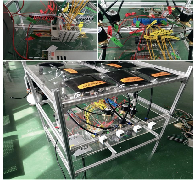
FIGURE 16: Model of a pneumatic device controlled by PLC.
