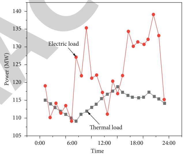
FIGURE 6: Typical daily load curve of electric load and heat load.
