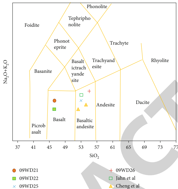
FIGURE 1: Diagram of the main element silico-alkali.
