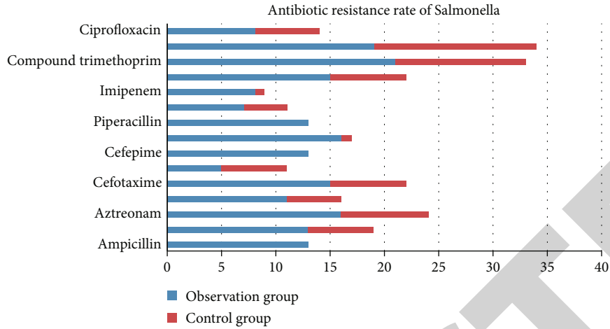
FIGURE 1: Antibiotic resistance rate of Salmonella.
