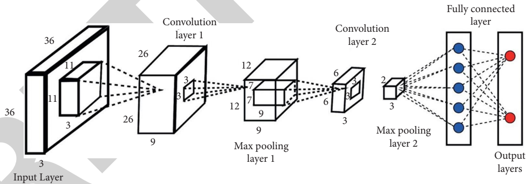
FIGURE 6: Architecture of a CNN.
