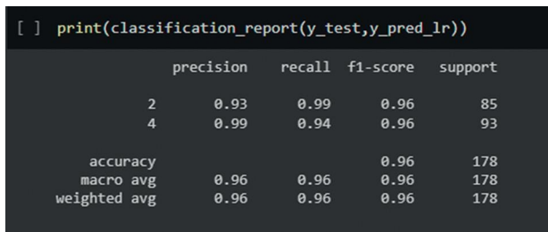
FIGURE 11: Classification result of logistic regression model.
