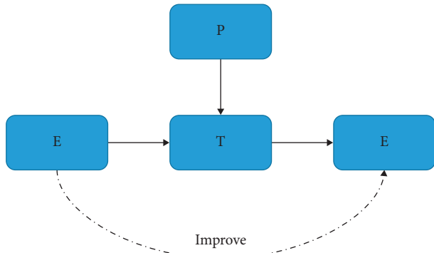
FIGURE 2: Learning algorithm.
