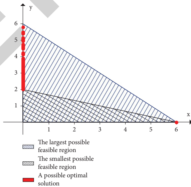
FIGURE 3: The set A and set B.
