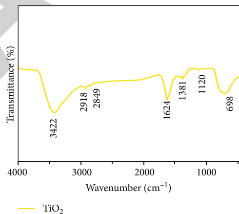
FIGURE 6: Biosynthesized \text{TiO}_2 nanoparticle FT-IR spectrum.
