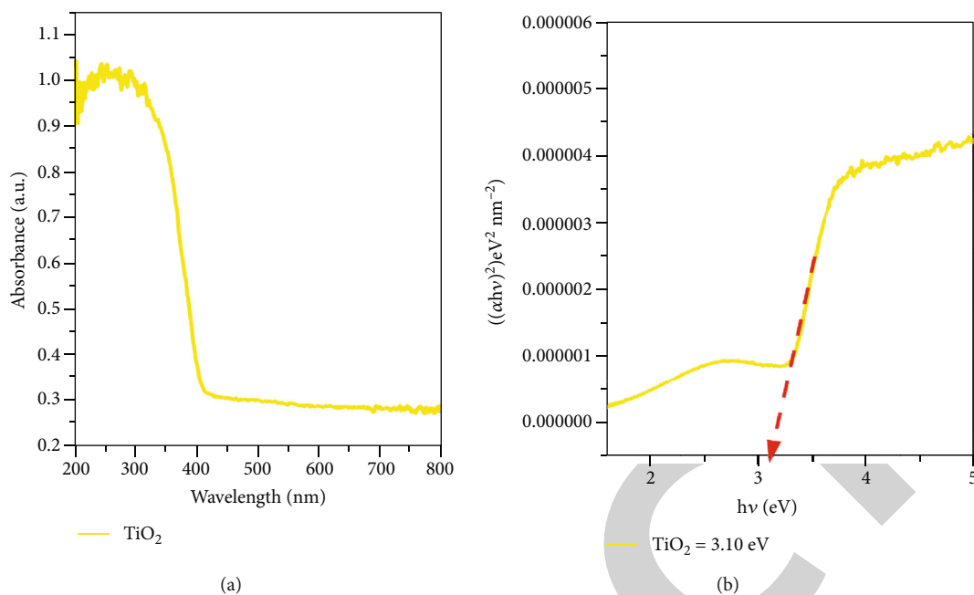
FIGURE 5: (a) Spectrum of UV-DRS absorption of biosynthesized \text{TiO}_2 NPs. (b) Synthesized NPs.
