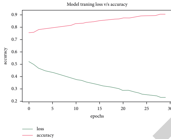
FIGURE 4: MLSTM_3 model accuracy and training loss plot.
