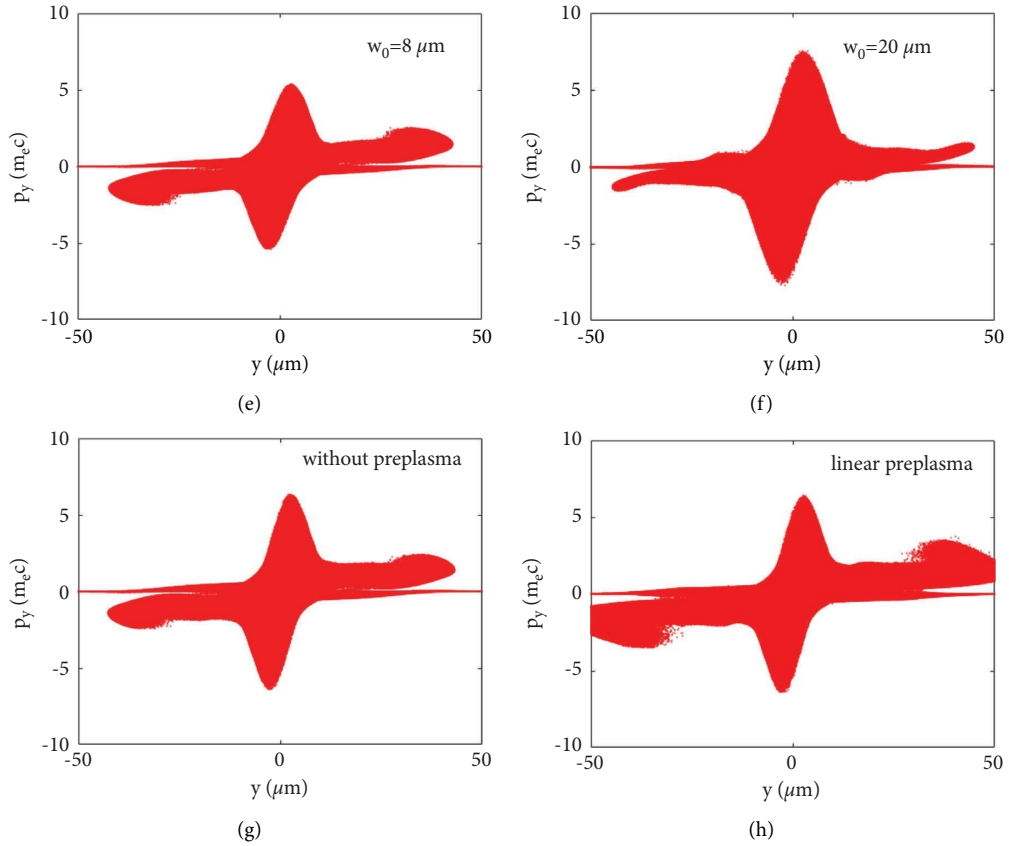
FIGURE 5: Electron momentum distribution with respect to laser intensity of (a) 3 \times 10^{19} \text{W/cm}^2 and (b) 1.2 \times 10^{20} \text{W/cm}^2 , plasma density of (c) 6 \times 10^{17} \text{cm}^{-3} and (d) 2.4 \times 10^{18} \text{cm}^{-3} , and laser focal spot size of (e) 8 \mu\text{m} and (f) 20 \mu\text{m} (g) without consideration of preplasma and (h) linear increasing preplasma at 78T_0 .
