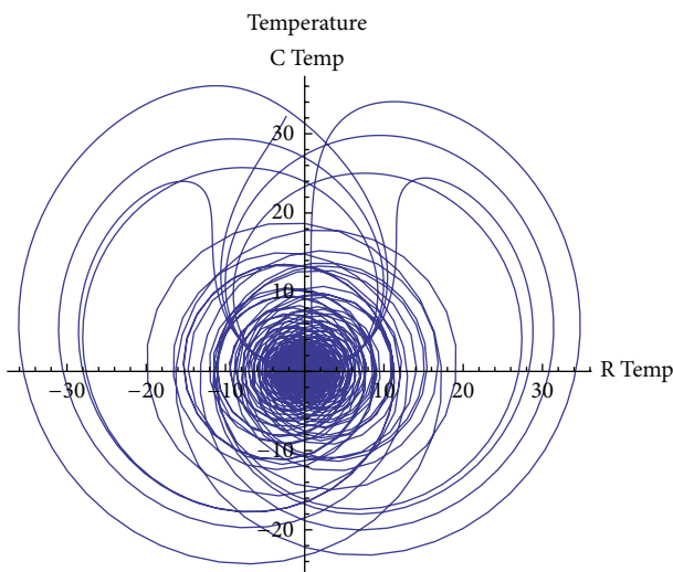
FIGURE 3: A chaotic global attractor of real and complex temperature for \varepsilon = 10 , B = 50 , \nu = 0 .
