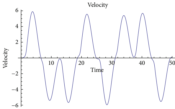
FIGURE 2: The inconsistent behavior of velocity for \varepsilon = 10 , B = 50 , \nu = 0 .
