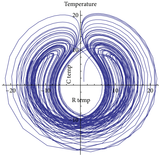
FIGURE 8: The chaotic but periodic plot of real and complex temperature for \varepsilon = 0.0001 , B = 40 , \nu = 0 .
