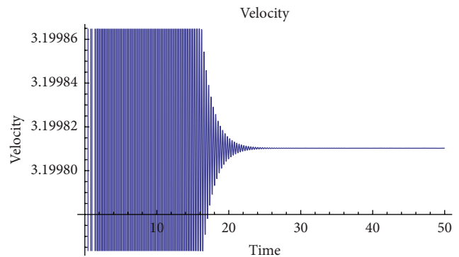
FIGURE 5: Velocity stabilizes at 3.19981 for \varepsilon = 0.1 , B = 100 , \nu = 0 .
