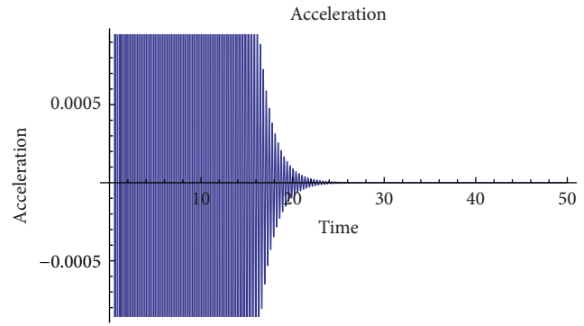
FIGURE 4: The stabilizing progress of acceleration for \varepsilon = 0.1 , B = 100 , \nu = 0 .
