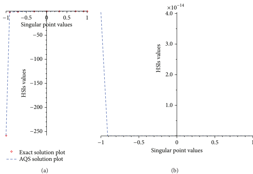
FIGURE 5: (a) Exact and AQS solutions when N = 40 and h(t) = 1/(2 + t) and (b) absolute error between exact and AQS solution when N = 40 and h(t) = 1/(2 + t) .
