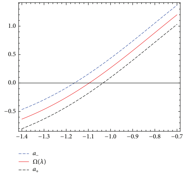
FIGURE 7: The enclosure interval dominating \lambda_{-1} for h = 0.2 , N = 25 , and \varepsilon = 10^{-2} .
