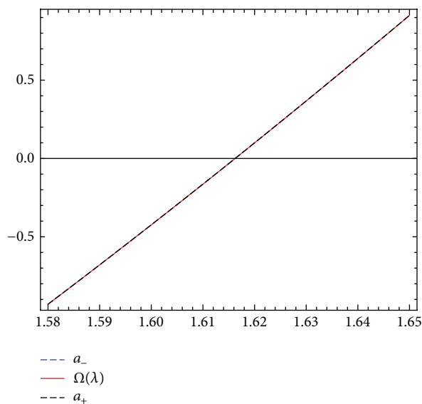
FIGURE 4: The enclosure interval dominating \lambda_1 for h = 0.1, N = 25 , and \varepsilon = 10^{-5} .
