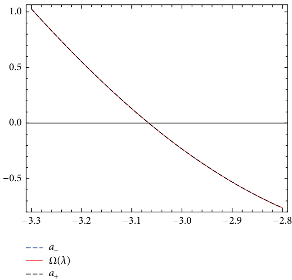
FIGURE 6: The enclosure interval dominating \lambda_{-2} for h = 0.2 , N = 25 , and \varepsilon = 10^{-5} .
