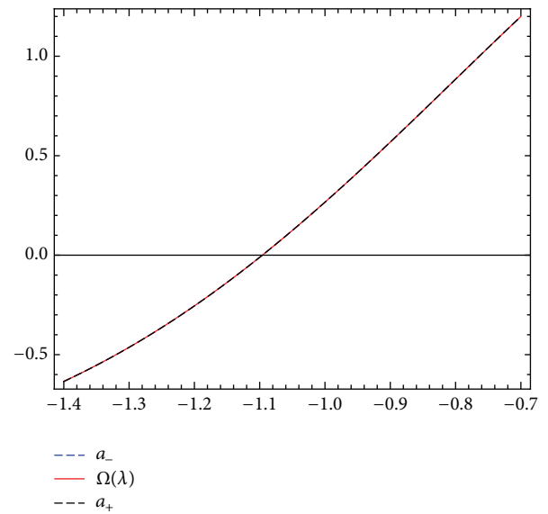
FIGURE 8: The enclosure interval dominating \lambda_{-1} for h = 0.2 , N = 25 , and \varepsilon = 10^{-5} .
