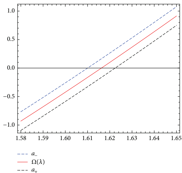
FIGURE 3: The enclosure interval dominating \lambda_1 for h = 0.1, N = 25 , and \varepsilon = 10^{-2} .
