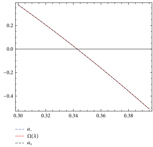
FIGURE 2: The enclosure interval dominating \lambda_0 for h = 0.1, N = 25, and \varepsilon = 10^{-5} .
