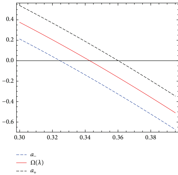
FIGURE 1: The enclosure interval dominating \lambda_0 for h = 0.1, N = 25, and \varepsilon = 10^{-2} .
