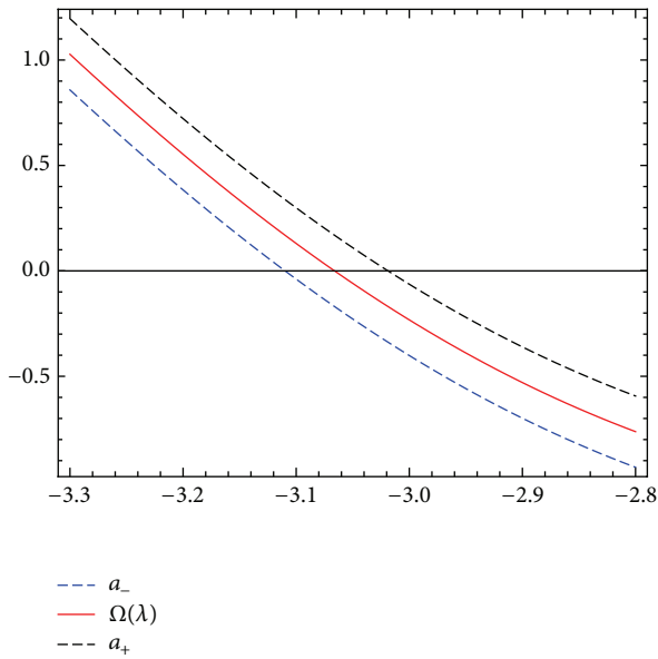
FIGURE 5: The enclosure interval dominating \lambda_{-2} for h = 0.2 , N = 25 , and \varepsilon = 10^{-2} .
