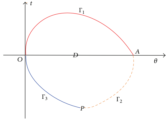
FIGURE 1: The domain D and its boundary in the formulations of the Tricomi problem.
