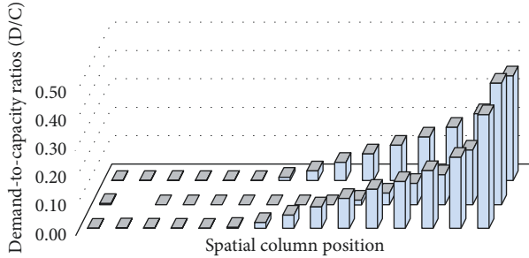
FIGURE 12: Demand to capacity ratios D/C: uneven distribution of inelastic response, CM placed with 14% of eccentricity in order to obtain \delta_{max}/\delta_{avg} = 1.4 in the equivalent linear static analysis.
