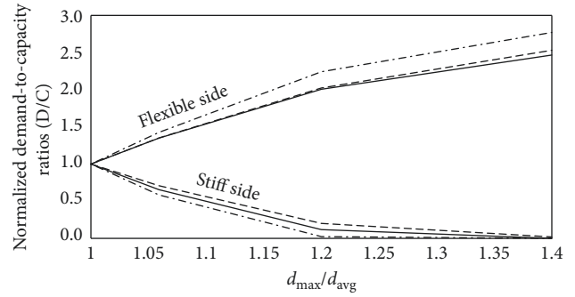
FIGURE 14: Normalized demand to capacity ratios D/C, calculated by means of nonlinear dynamic analyses, at varying \delta_{max}/\delta_{avg} provided by equivalent linear static analysis. Comparison between the inelastic response of the column placed on the stiff side and that provided by the column on the flexible side.
