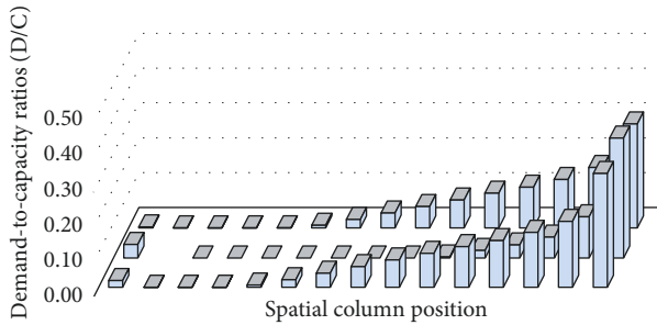
FIGURE 11: Demand to capacity ratios D/C: uneven distribution of inelastic response, CM placed with 6% of eccentricity in order to obtain \delta_{max}/\delta_{avg} = 1.2 in the equivalent linear static analysis.
