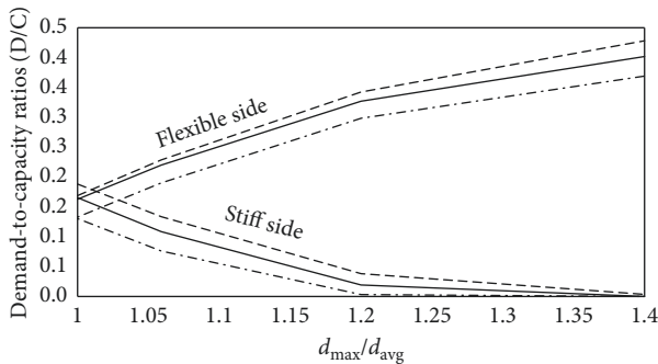
FIGURE 13: Demand to capacity ratios D/C, calculated by means of nonlinear dynamic analyses, at varying \delta_{max}/\delta_{avg} provided by equivalent linear static analysis. Comparison between the inelastic response of the column placed on the stiff side and that provided by the column on the flexible side.
