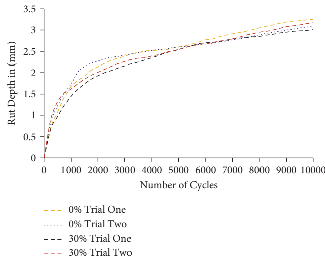
FIGURE 13: Rutting test result of control mix and 30% Belessa kaolin.
